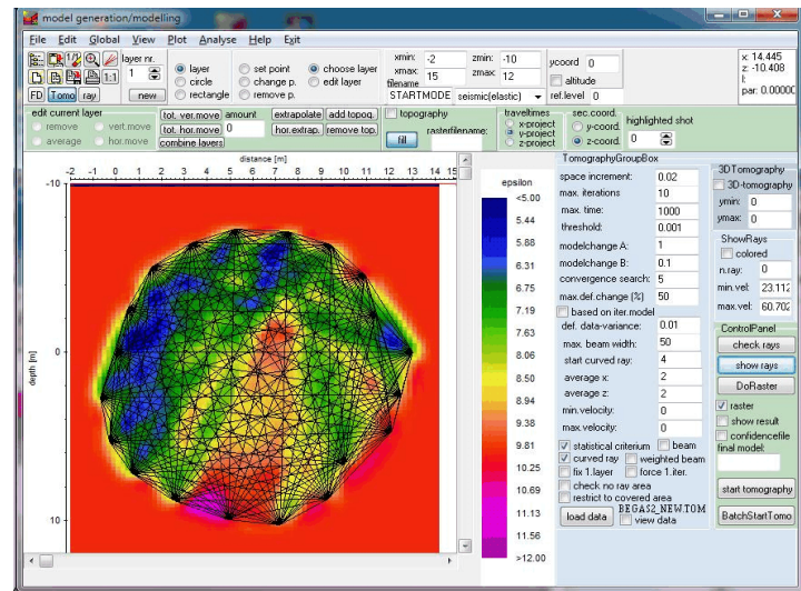
example of a tomographic inversion for a cylindrical object
