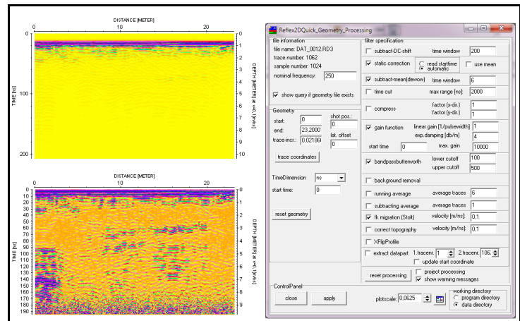
Comparison of the original raw data (upper panel) with the processed data (lower panel) based on the settings given in the right geometry_processing menu.
