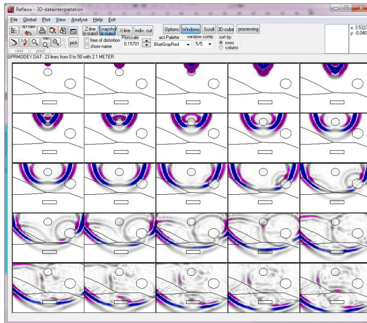
Snapshot sequence for a point source - 25 snapshots bewtween 0 and 50 ns are shown
