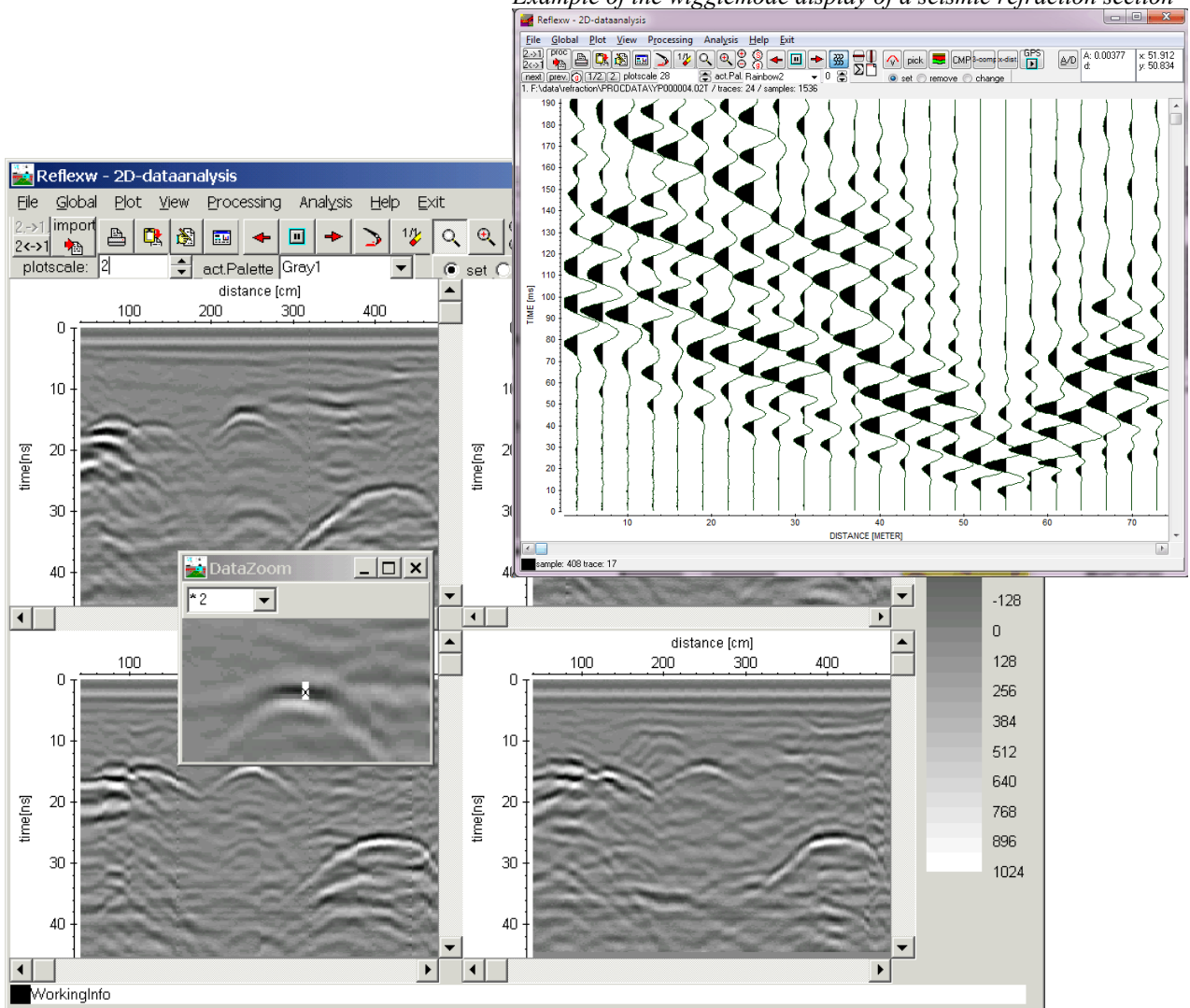
Example of the pointmode display of 4 different GPR-lines with activated magnifying glass
