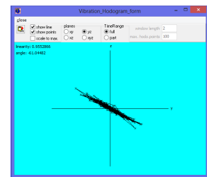
Hodogram: Same Data shown in y-z-plane
