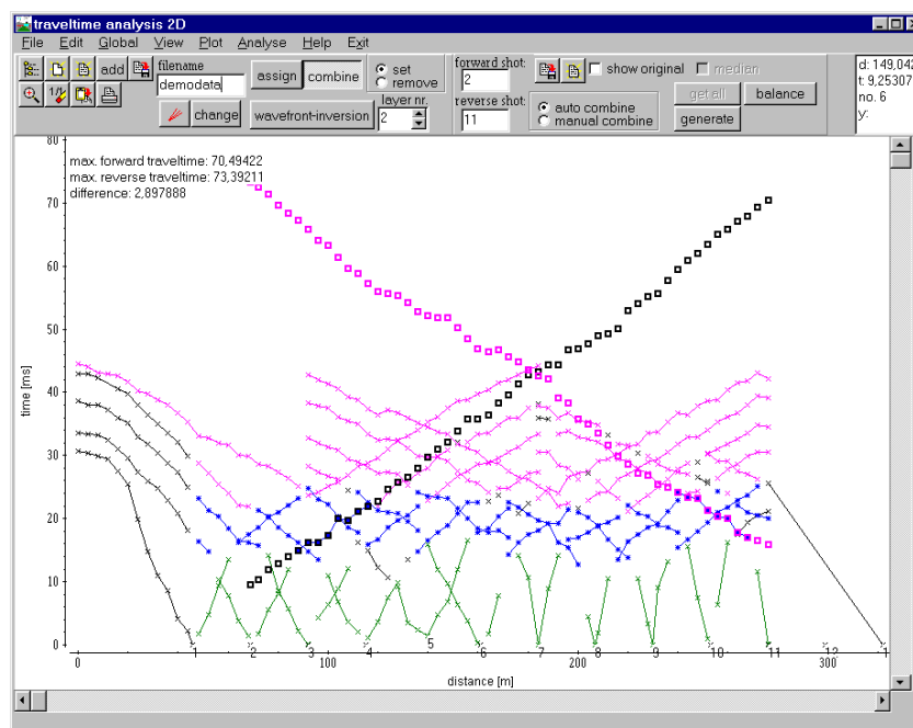
Traveltime data put together and assigned to 3 different layers - for layer 2 one complete forward and reverse traveltime curve has been automatically generated which is the basis for a subsequent wavefront inversion
